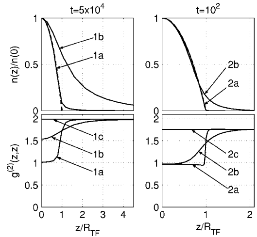
FIG. 7. Density profiles n(z)/n(0) and the local pair correlation g^{(2)}(z, z) as a function of z/R_{TF} for a harmonically trapped 1D Bose at different temperatures t : t=5 \times 10^4 (first column) and 10^2 (second column). The values of the interaction parameter \gamma(0) in the trap center for each of the curves are as follows: 1a, \gamma(0)=1.57 \times 10^{-4} ; 1b, \gamma(0)=1.14 \times 10^{-3} ; 1c, \gamma(0)=0.196 ; 2a, \gamma(0)=1.65 \times 10^{-3} ; 2b, \gamma(0)=2.31 \times 10^{-2} ; and 2c, \gamma(0)=6.30 . The dashed lines represent the Thomas-Fermi inverted parabola Eq. (3.13). The density profiles corresponding to the lower-density cases 1c and 2c are well approximated by the thermal (Gaussian) distribution for a classical ideal gas, Eq. (4.4), and are omitted from the graphs for clarity. The respective pair correlations for these low-density cases are almost constant along the entire sample and are given by the value of g^{(2)}(z, z) in the tails of the distribution z \rightarrow \infty . Depending on the temperature t , these values can be determined using the results of Fig. 5 at \gamma(z) \gg 1 [see the curve for \gamma(z)=50 ].
