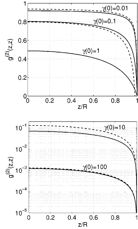
FIG. 2. The local pair correlation of a trapped 1D Bose gas at zero temperature, g^{(2)}(z, z) , as a function of the displacement from the trap center, z/R , for different values of \gamma(0) . The full lines are the results of numerical calculation, while the dashed lines for \gamma(0) = 0.01, 0.1 and \gamma(0) = 10, 100 are the respective analytic results of Eqs. (3.12) and (3.16) shown for comparison.
