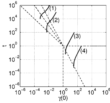
FIG. 9. Diagram of the regimes of a trapped 1D Bose gas as in Fig. 3, except that the curved lines (1)–(4) represent the locations of the interaction parameter \gamma(0) and the reduced temperature t , for four different (fixed) values of the global interaction parameter \tilde{\gamma} while the global temperature \theta is changing. This represents four different samples with fixed total number of particles N and varying absolute temperature T . For each point on a given line, there exists an associated density profile with the peak density n(0) corresponding to the respective value of \gamma(0) , and the local values n(z) corresponding to the values of \gamma(z) in the horizontal direction to the right. The values of the global interaction parameter \tilde{\gamma} for each line are (1) 0.002, (2) 0.01, (3) 1, and (4) 10.
