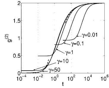
FIG. 5. Local pair correlation g^{(2)} as a function of the reduced temperature t , for different values of the interaction parameter \gamma . The solid lines are the exact numerical results, while the dashed lines correspond to the approximate analytic result of Eq. (5.12).
