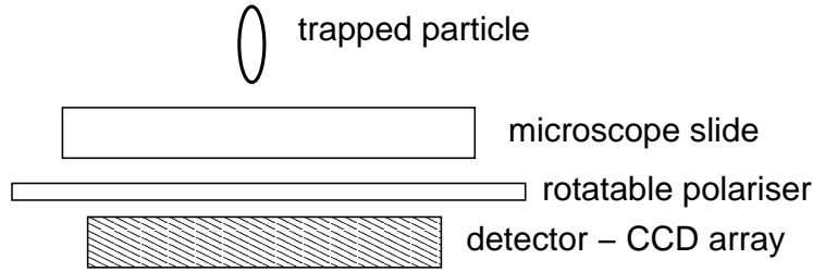
Fig. 4. Using a polariser and CCD array to measure the polarisation state of light scattered by a trapped particle
