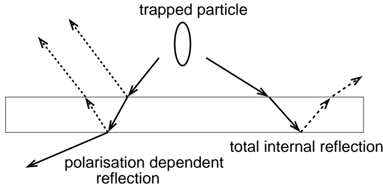
Fig. 5. Total internal limits the maximum angle at which light can be scattered and still exit the trapping cell
