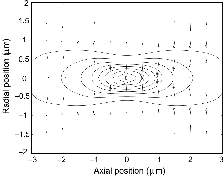
Fig. 2. Optical force on spheroid
