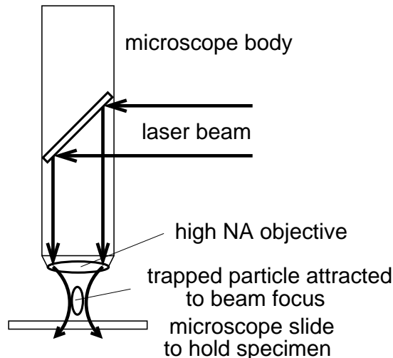
Fig. 1. Schematic diagram of a typical optical tweezers setup
