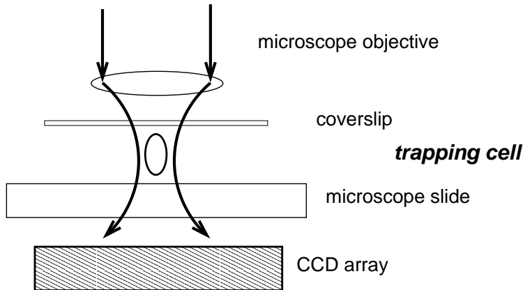
Fig. 3. Optical trap with a CCD array to measure scattered light
