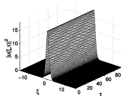
FIG. 9. Exact soliton dynamics with the exact solitary solution (found numerically) as the initial condition, for \alpha_{11}=0.1 , \gamma=1 , and N^l being fixed to the same value as in the respective GVA solution. Shown is the particle number density for the atomic field, with similar behavior found for the molecular field.
