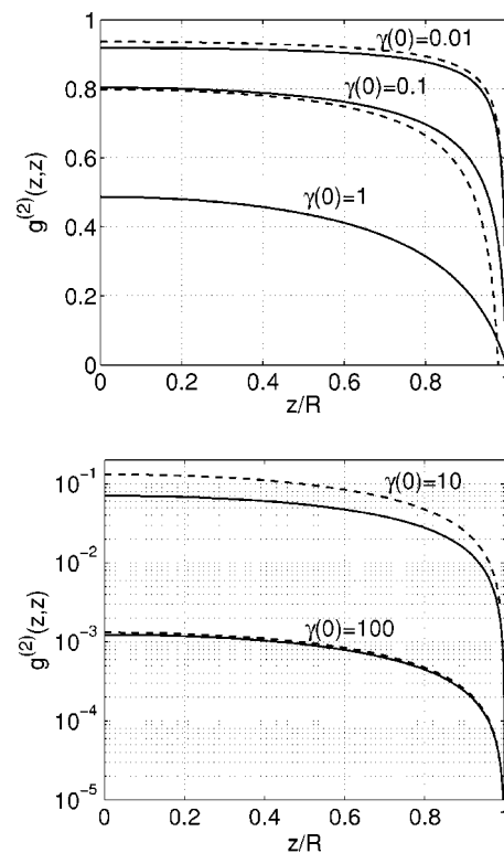
FIG. 2. The local pair correlation of a trapped 1D Bose gas at zero temperature, g^{(2)}(z,z) , as a function of the displacement from the trap center, z/R , for different values of \gamma(0) . The full lines are the results of numerical calculation, while the dashed lines for \gamma(0)=0.01, 0.1 and \gamma(0)=10, 100 are the respective analytic results of Eqs. (3.12) and (3.16) shown for comparison.
