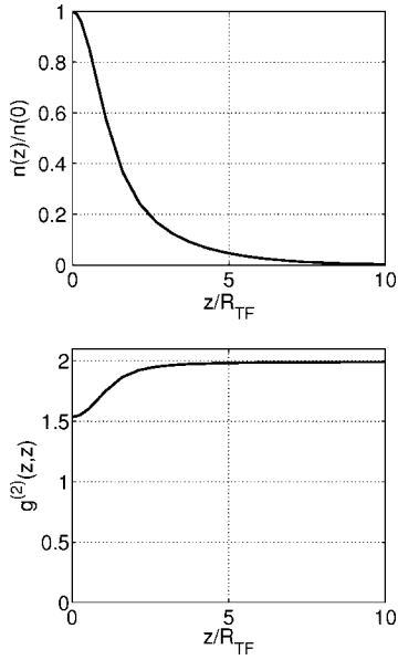
FIG. 4. Density profile n(z)/n(0) and the local pair correlation g^{(2)}(z,z) as a function of the distance from the trap center z/R_{TF} , for T=0.2T_Q ( t=5 \times 10^4 ) and \gamma(0)=1.14 \times 10^{-3} . This corresponds to case 1b in the diagram of Fig. 6 below.
