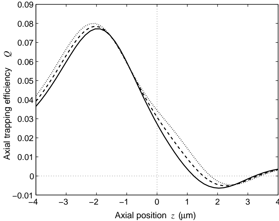
Figure 3: Axial trapping efficiency. The trapping efficiency is shown for an oblate spheroidal chloroplast with semi-minor axis 0.5 \mu\text{m} and semi-major axes 2 \mu\text{m} . The trapping efficiency is shown for chloroplasts aligned along the beam axis, at varying angles to the plane of polarisation. The force is shown for chloroplasts aligned with the plane of polarisation (solid line), at 45^\circ to (dashed line), and perpendicular to the plane of polarisation (dotted line). The equilibrium position in all cases is with the centre of the chloroplast slightly beyond the focal plane of the beam located at z = 0 .
